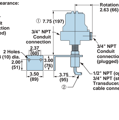
Remote Mount with Guarded Probe
