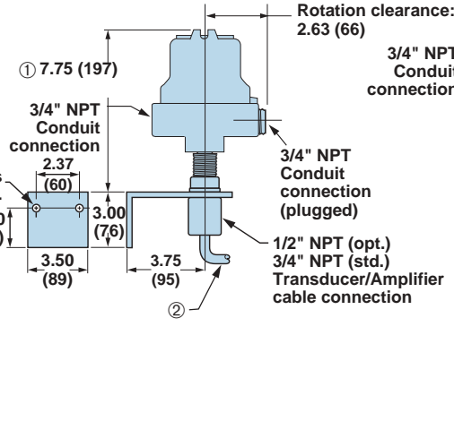
Remote Mount with Standard Rigid Probe
