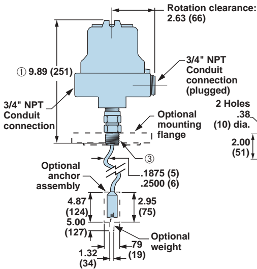
Integral Mount with Flexible Probe
